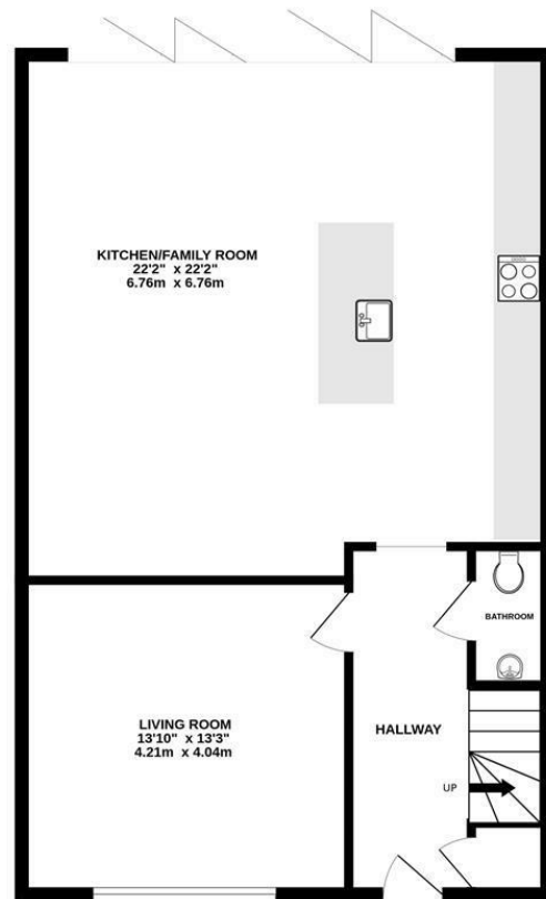
GROUND FLOOR 786 sq.ft. (73.0 sq.m.) approx.
