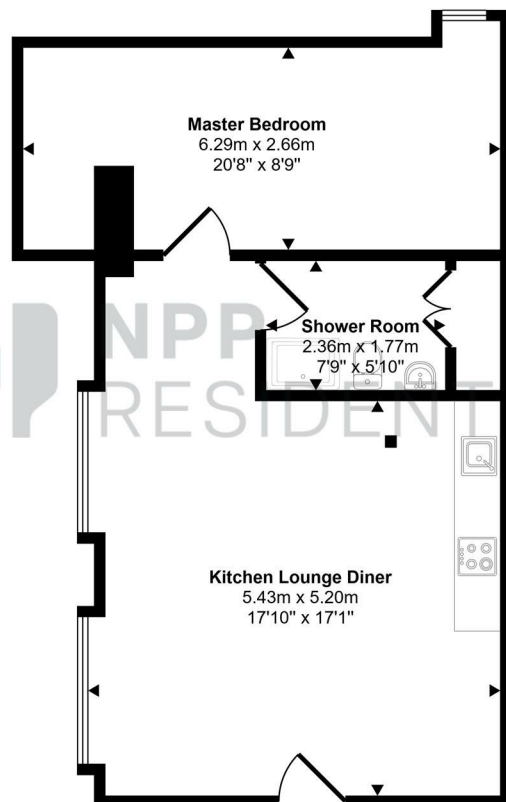
Floorplan
