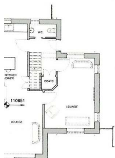
Ground floor- new dwelling
