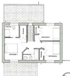
First floor- New dwelling 1 : 100
