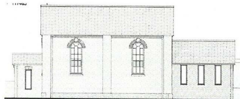
SW elevation- Proposed conversion 1 : 100
