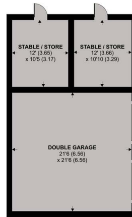
OUTBUILDING / GARAGE 1 / 2
