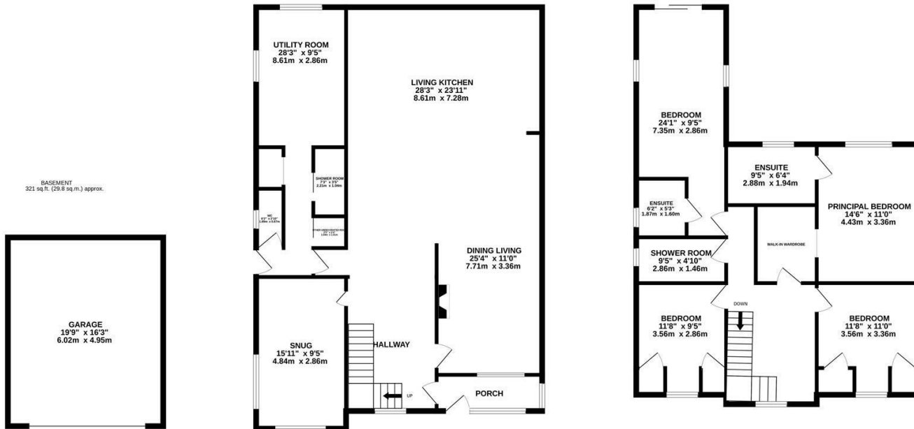
GROUND FLOOR 1275 sq.ft. (118.5 sq.m.) approx.
