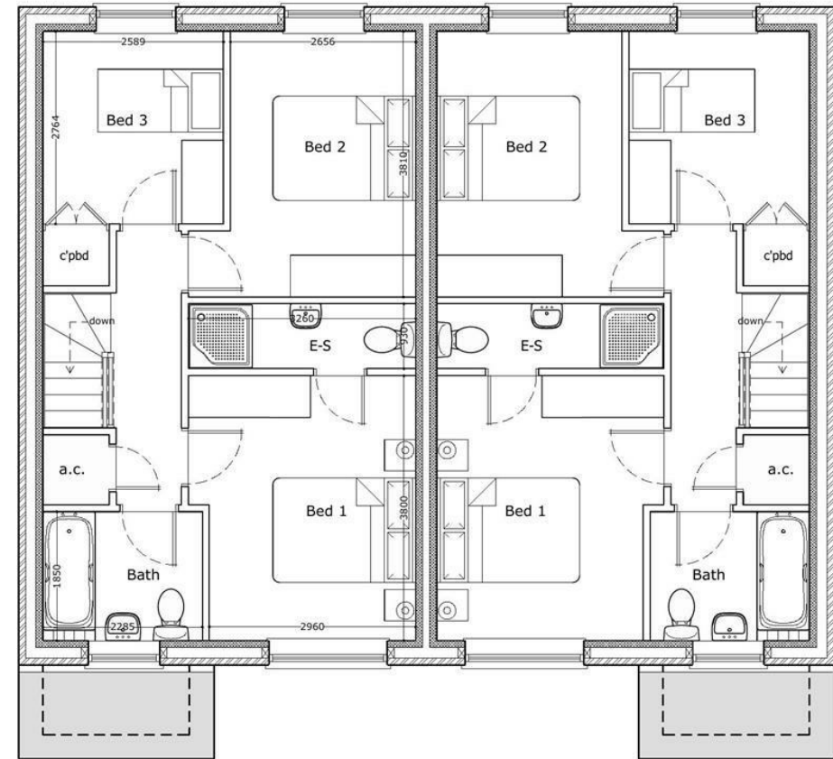
Proposed First Floor Plans
