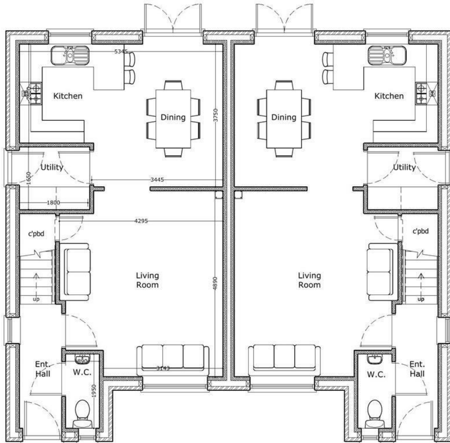
Proposed Ground Floor Plans Gross Floor Area = 96m 2 or 1033ft 2
