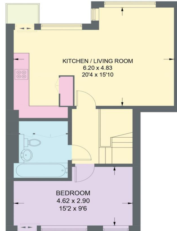
TENTH FLOOR 53.8 SQ M / 579 SQ FT
