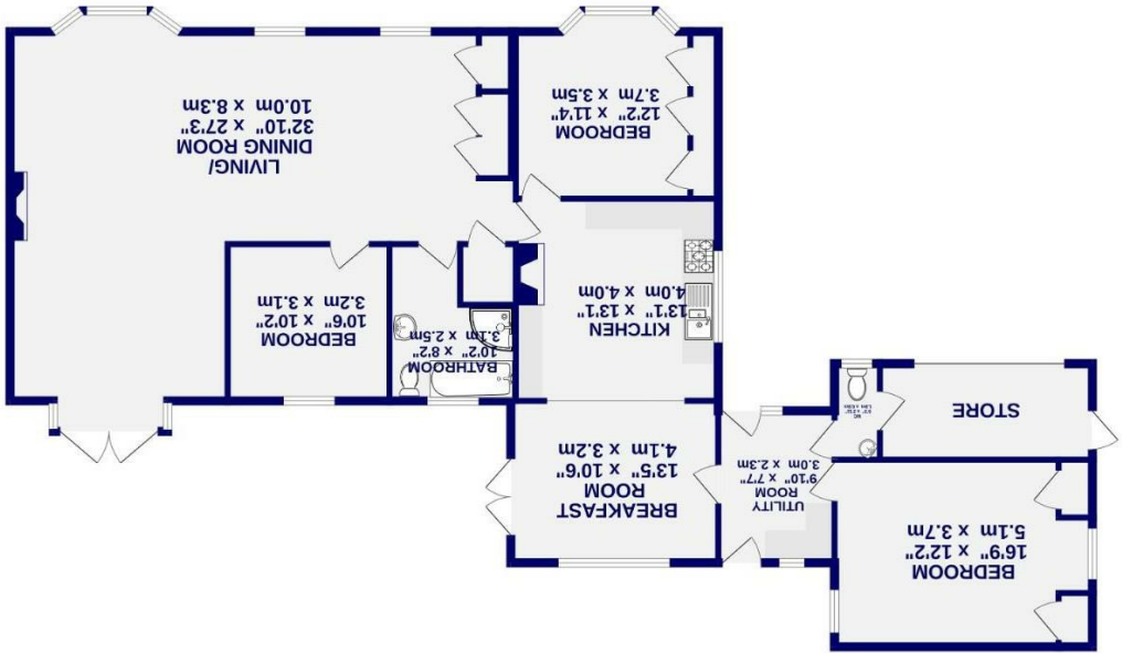
GROUND FLOOR 1644 sq.ft. (152.8 sq.m.) approx.
