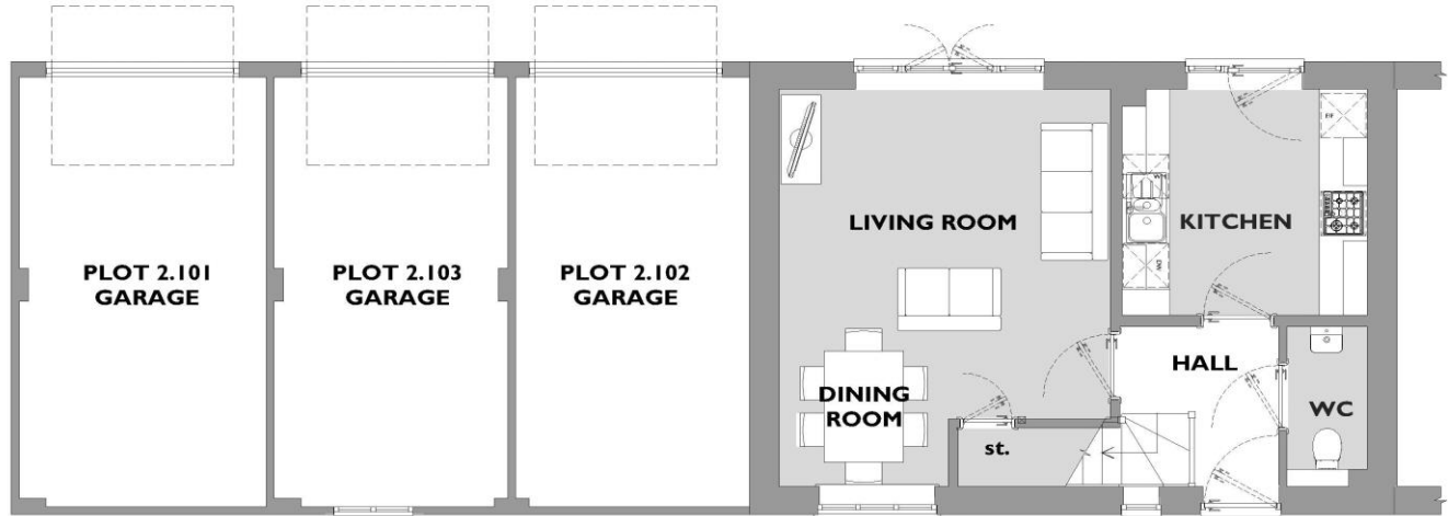
GROUND FLOOR
