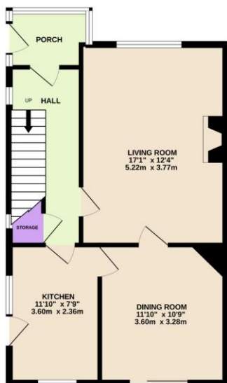
GROUND FLOOR 544 sq.ft. (50.6 sq.m.) approx.
