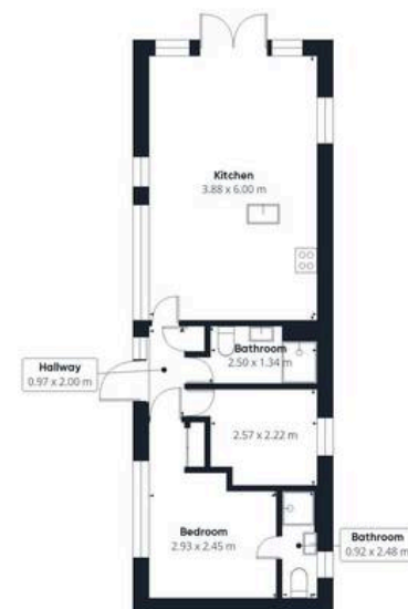
Floor 0 Building 2
