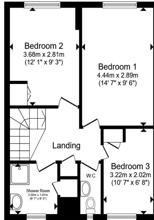
Second Floor
