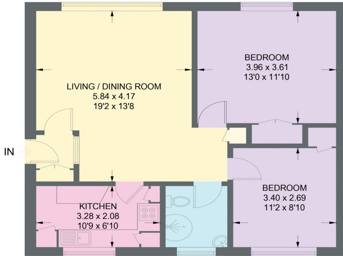
FIRST FLOOR
