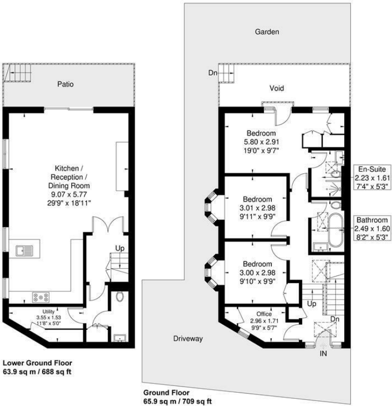
Ashfield Road Approximate Gross Internal Area = 129.8 sq m / 1397 sq ft
