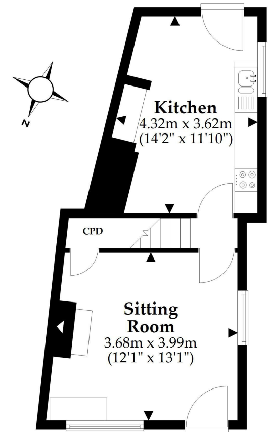
Ground Floor Approx. 31.2 sq. metres (335.9 sq. feet)
