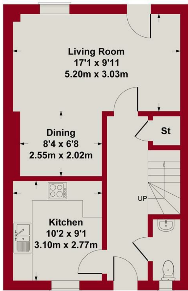
GROUND FLOOR
