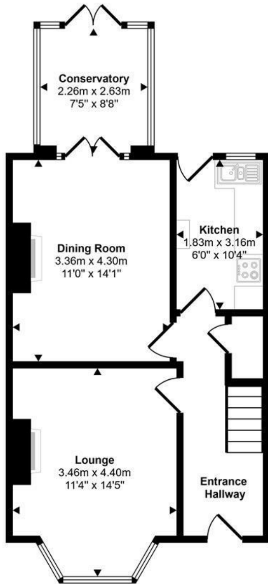
Ground Floor Approx 50 sq m / 540 sq ft
