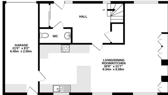
GROUND FLOOR 835 sq.ft. (77.6 sq.m.) approx.
