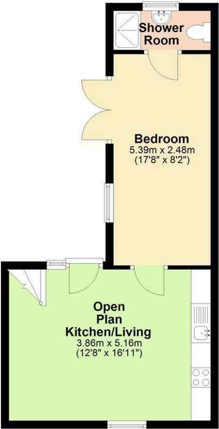
Ground Floor Approx. 36.3 sq. metres (390.7 sq. feet)
