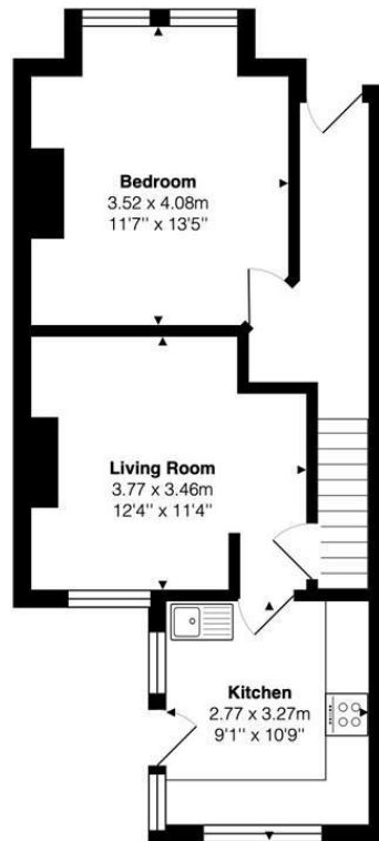
Lower Ground Floor Area: 42.4 m 2 ... 456 ft 2
