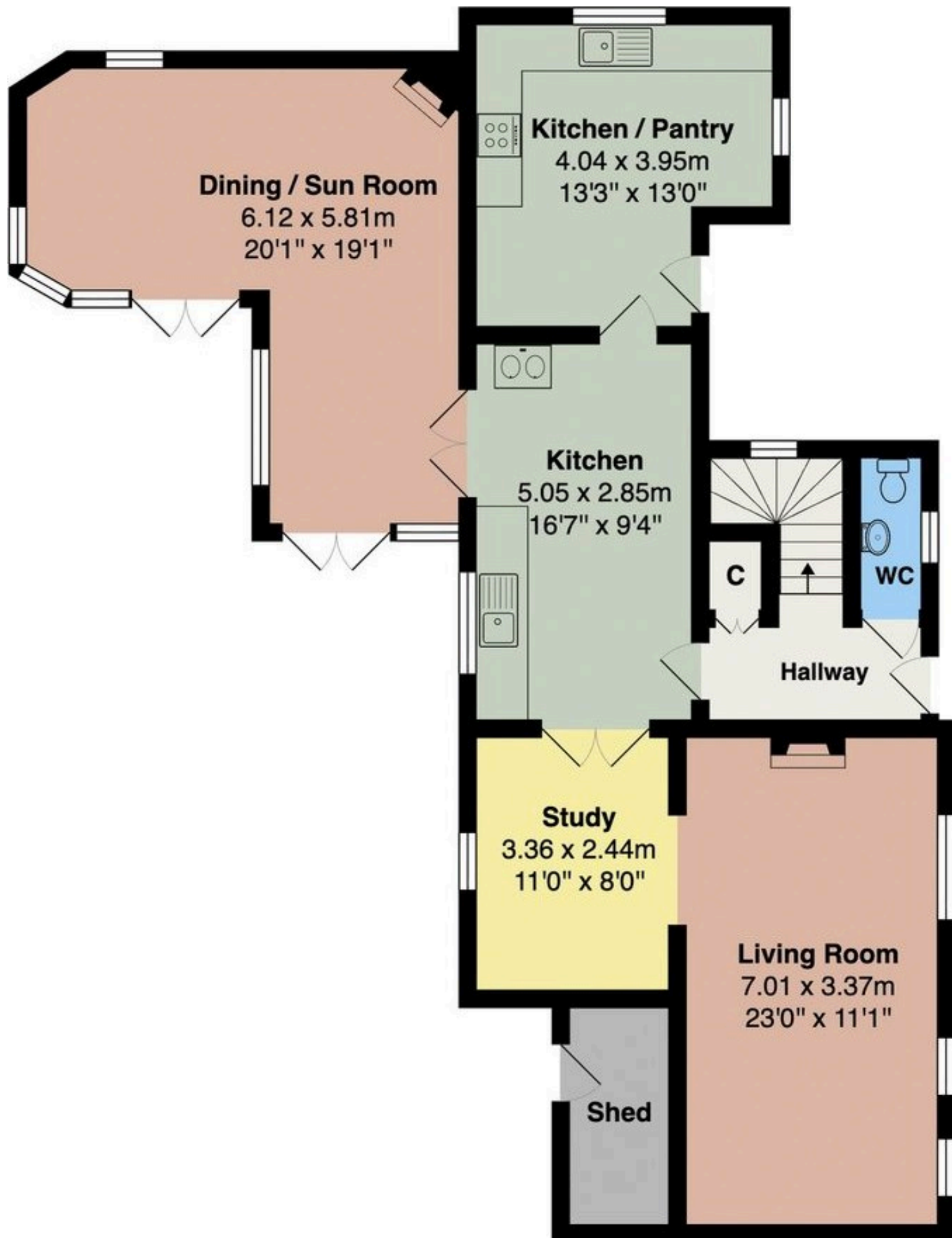
Ground Floor Area: 105.0 m 2 ... 1130 ft 2
