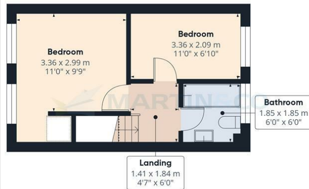
Floor 1 Building 1
