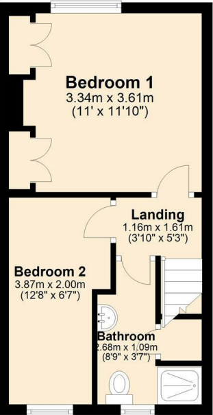
First Floor Approx. 26.4 sq. metres (284.2 sq. feet)
