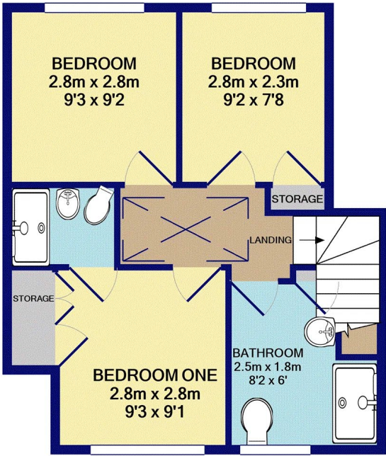
1ST FLOOR APPROX. FLOOR AREA 37.7 SQ.M. (406 SQ.FT.)
