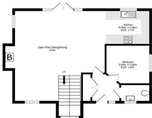
Ground Floor 58.9 sq.m. (634 sq.ft.) approx.
