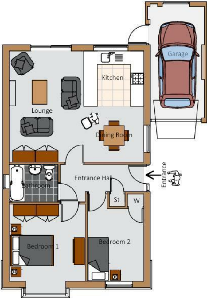
5 GROUND FLOOR scale nts
