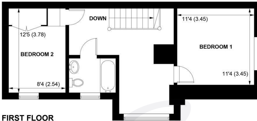
FIRST FLOOR
