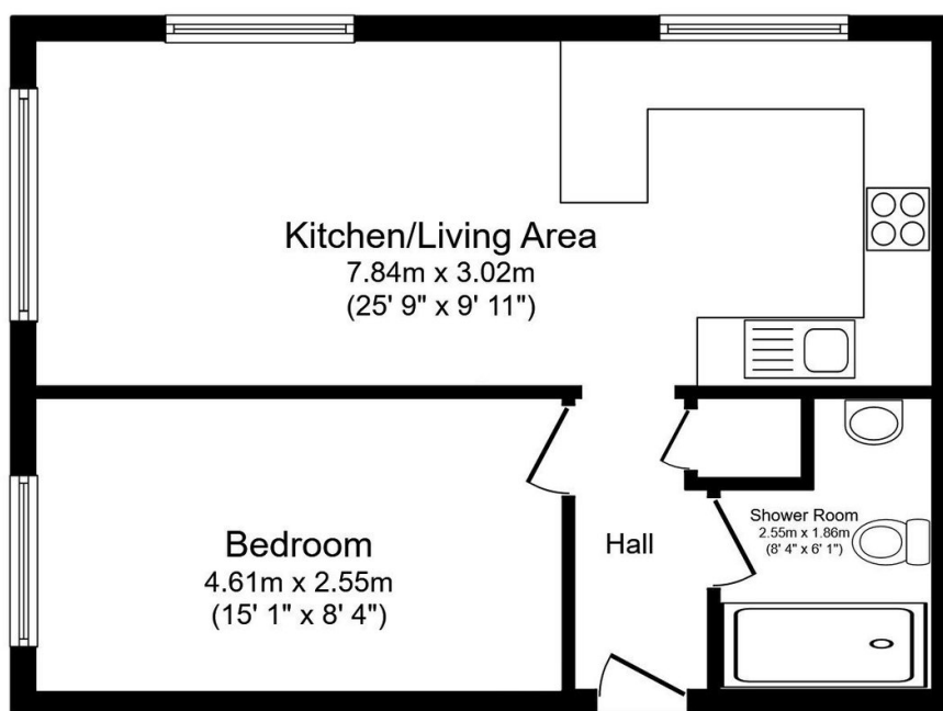
Floor Plan
