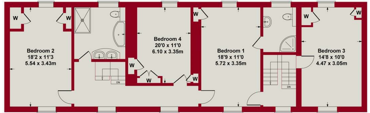
FIRST FLOOR
