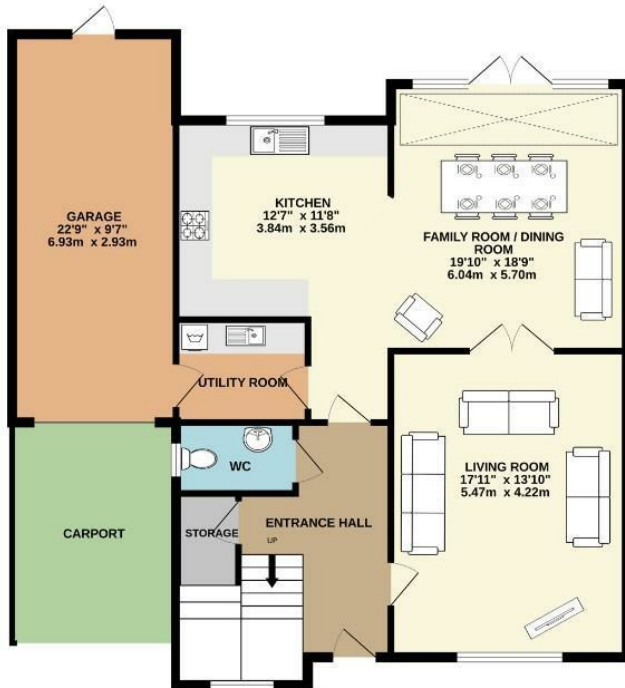
GROUND FLOOR 1,093 sq.ft. (101.5 sq.m.) approx.
