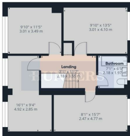
Floor 1 Building 1
