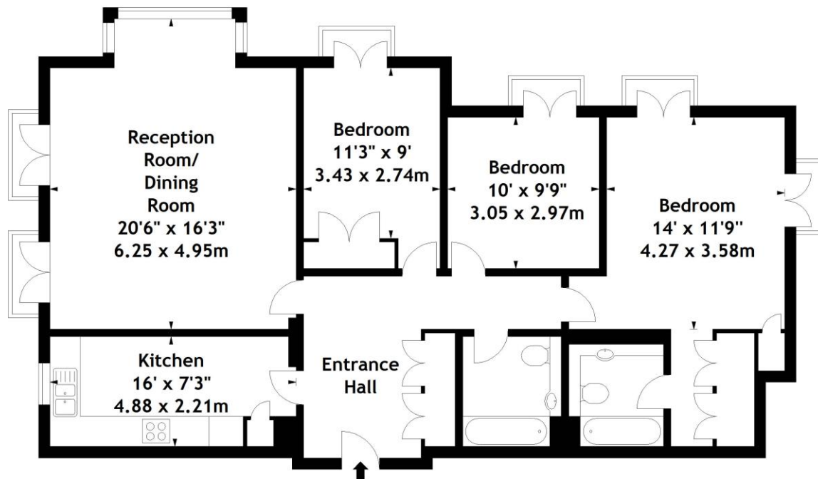
First Floor
