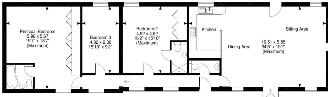
Ground Floor
