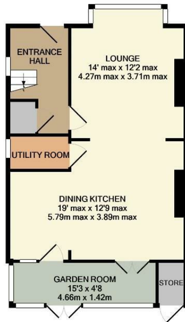
GROUND FLOOR APPROX. FLOOR AREA 549 SQ.FT. (51.0 SQ.M.)
