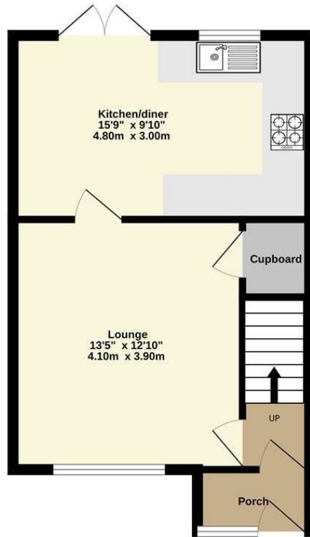
Ground Floor 391 sq.ft. (36.3 sq.m.) approx.
