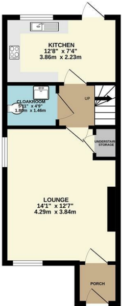
GROUND FLOOR 356 sq.ft. (33.1 sq.m.) approx.
