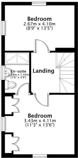
First Floor Approx. 35.5 sq. metres (381.9 sq. feet)
