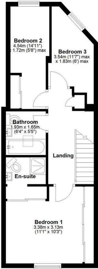
First Floor Approx. 41.6 sq. metres (448.0 sq. feet)
