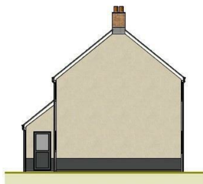
South East Elevation. Scale 1:100
