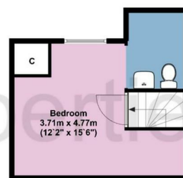
Second Floor Approx 21.00 Sq meters (226.00 Sq feet).
