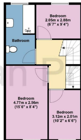
First Floor Approx 41.00 Sq meters (441.00 Sq feet).
