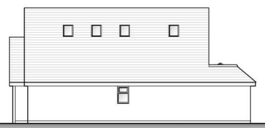
PROPOSED RIGHT SIDE ELEVATION
