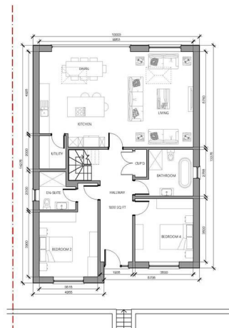
PROPOSED GROUND FLOOR PLAN 1:100
