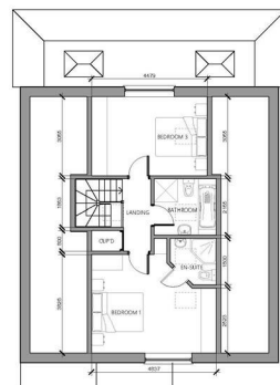
PROPOSED ROOF PLAN 1:100
