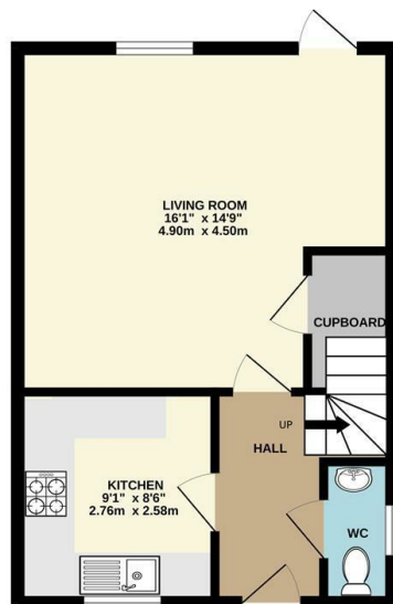
GROUND FLOOR 383 sq.ft. (35.6 sq.m.) approx.
