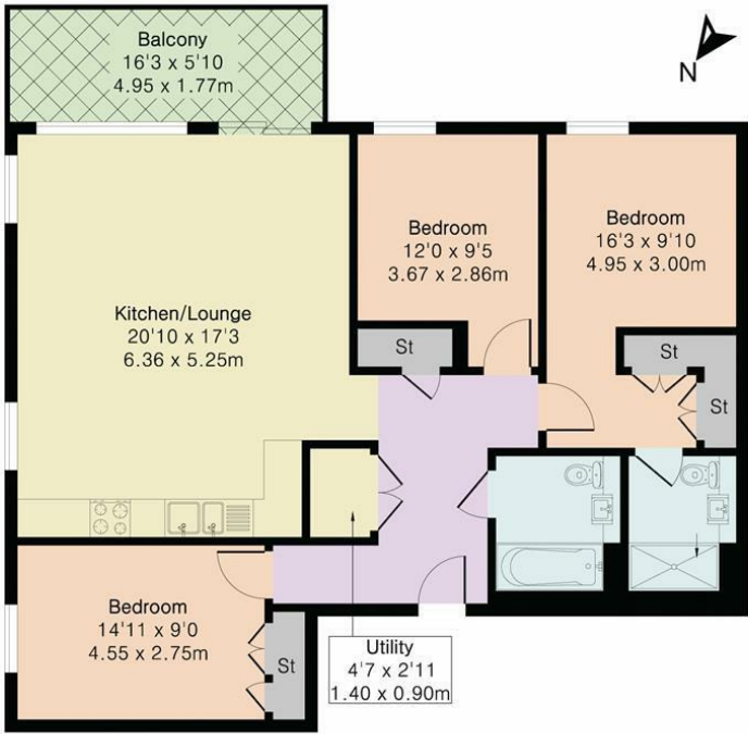
Fourth Floor
