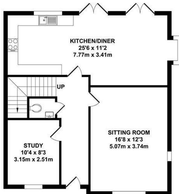
GROUND FLOOR APPROX. FLOOR AREA 709 SQ.FT. (65.86 SQ.M.)
