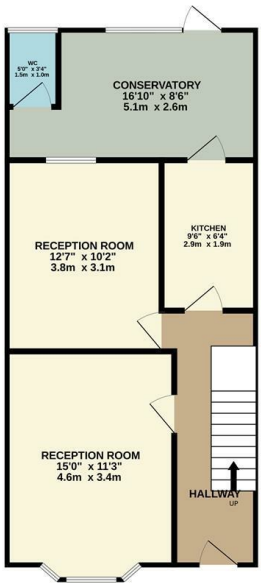
GROUND FLOOR 578 sq.ft. (53.7 sq.m.) approx.
