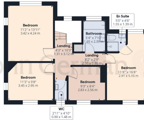
Floor 1 Building 1
