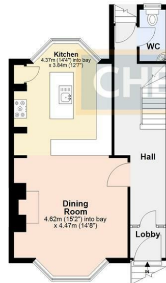
Upper Ground Floor Approx. 49.6 sq. metres (533.4 sq. feet)
