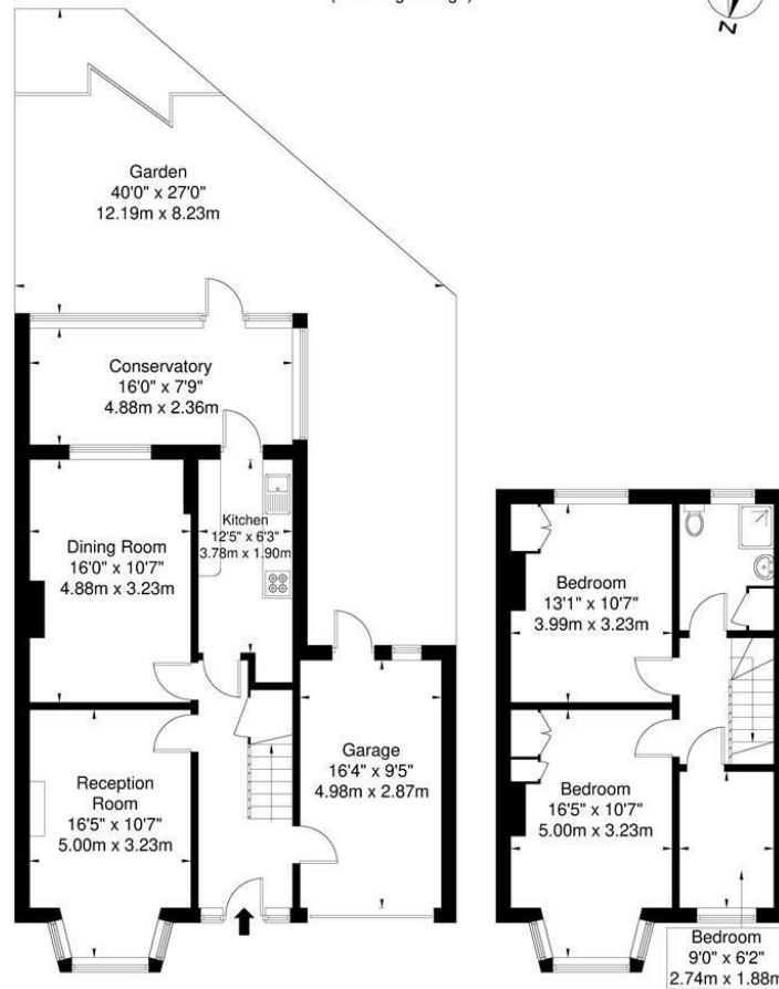
Ground Floor First Floor For Illustration Purposes Only - Not To Scale
