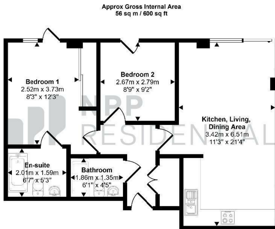
Floorplan
