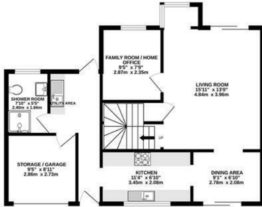
GROUND FLOOR 697 sq.ft. (64.7 sq.m.) approx.
